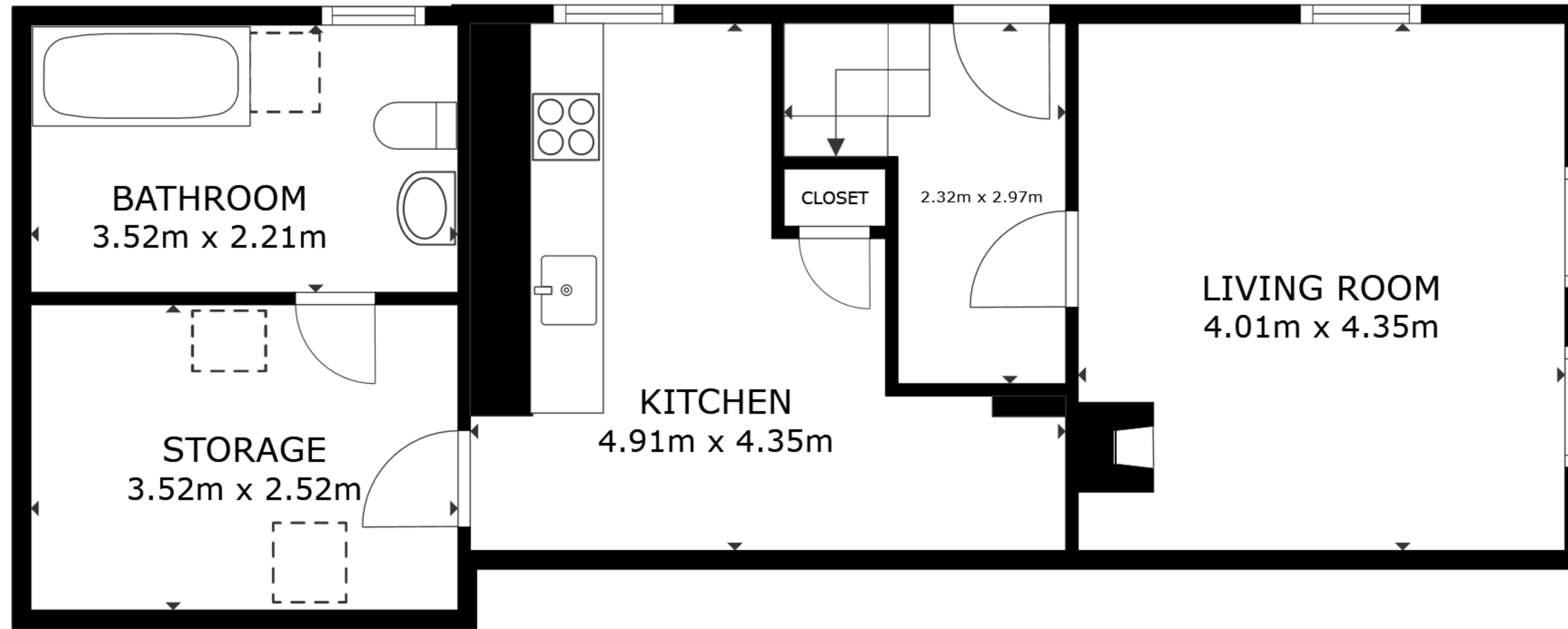
FLOOR 1
